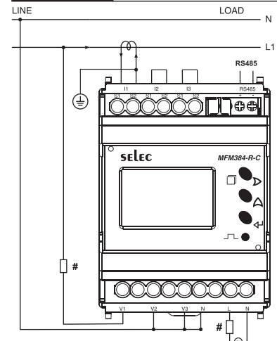
1 Phase - 2 Wire 1 Ø - 2 Wire, 1 CT
