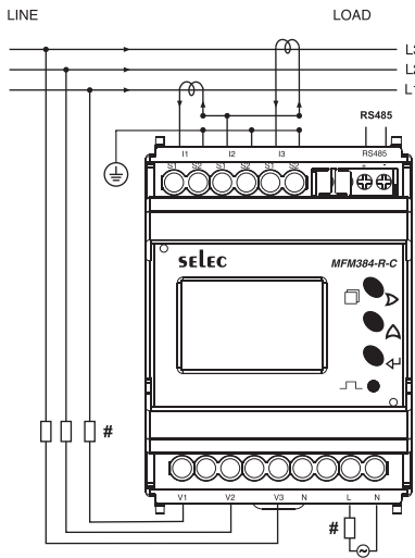
3 Phase - 3 Wire 3 Ø - 3 Wire, 2 CT'S
