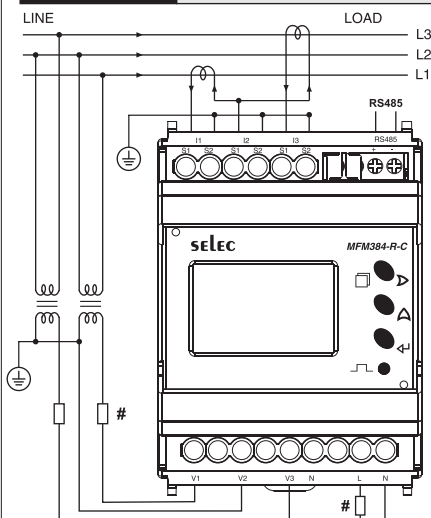
3 Phase - 3 Wire 3 Ø - 3 Wire, 2 CT'S and 2 PT'S
