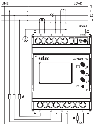
3 Phase-4 Wire (Commonly Used) 3 Ø - 4 Wire, 3 CT'S
